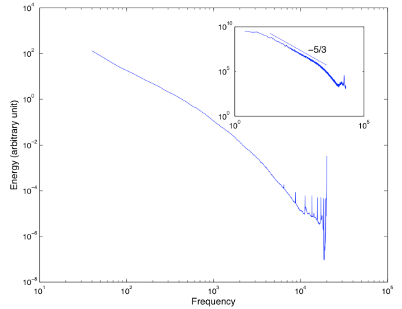
Figure 5: Hilbert marginal spectrum of the velocity signal. For comparison Fourier spectrum is displayed in the up-right panel.
